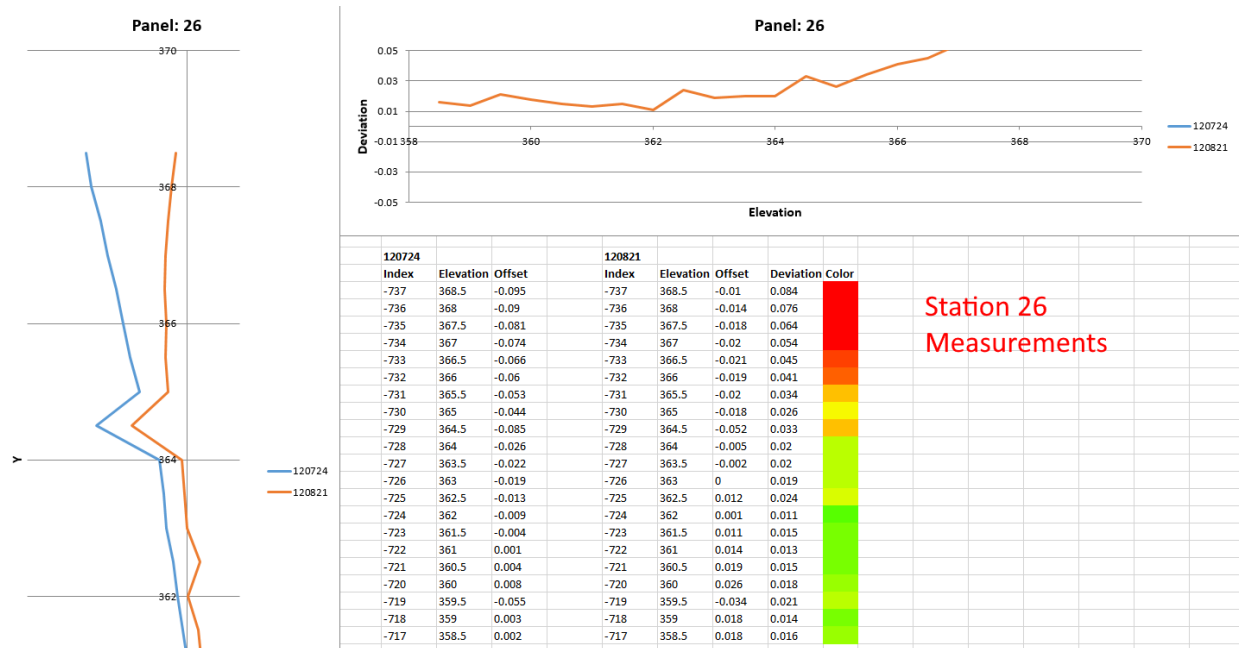
Figure 41: Individual Station Measurements Linked from Summary Page
