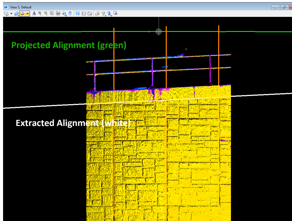
Figure 2: Evaluate panel data at equidistant spacing along horizontal alignment
