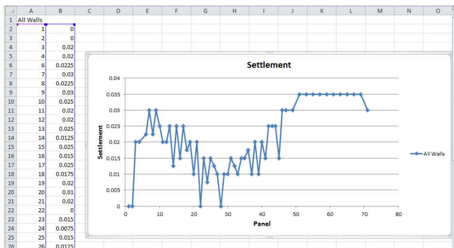
Figure 43: Settlement as measured by vertical movement of the joints at each station
