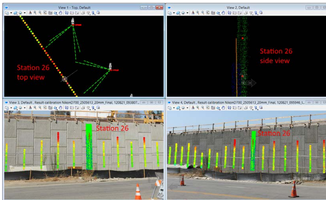
Figure 39: Information Rich TopoDOT Environment
