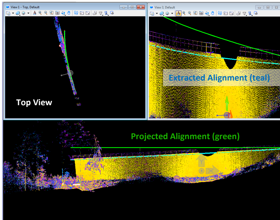
Figure 1: Baseline alignment extracted along edge of wall cap
