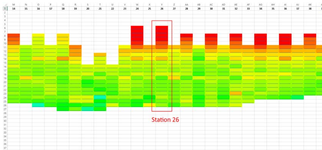
Figure 40: Wall Monitoring Summary Spread Sheet Shows Color-coded Movement at Every Station
