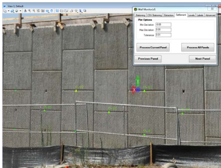
Figure 42: TopoDOT™ extracted settlement measurements projected onto joints
